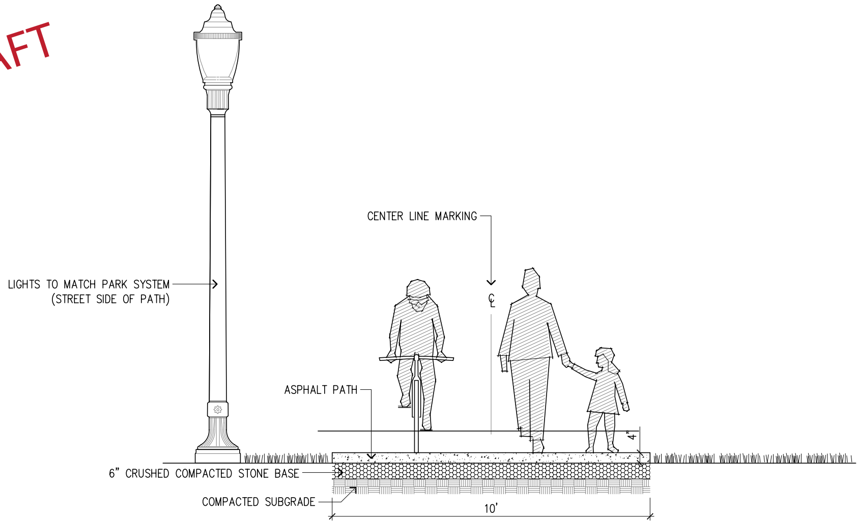
BICYCLE PATH TYP.
